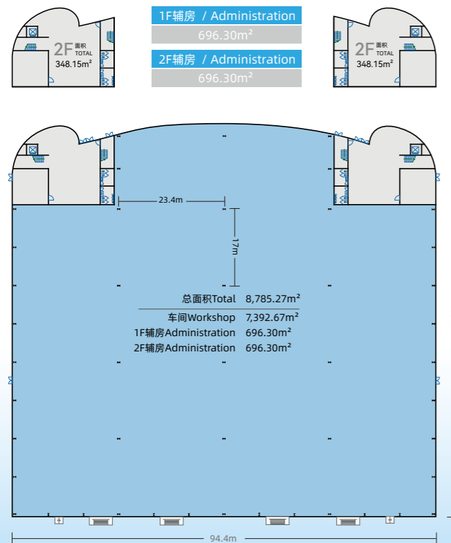
车间平面图(A9-A11) LAYOUT OF WORKSHOP (A9-A11)
