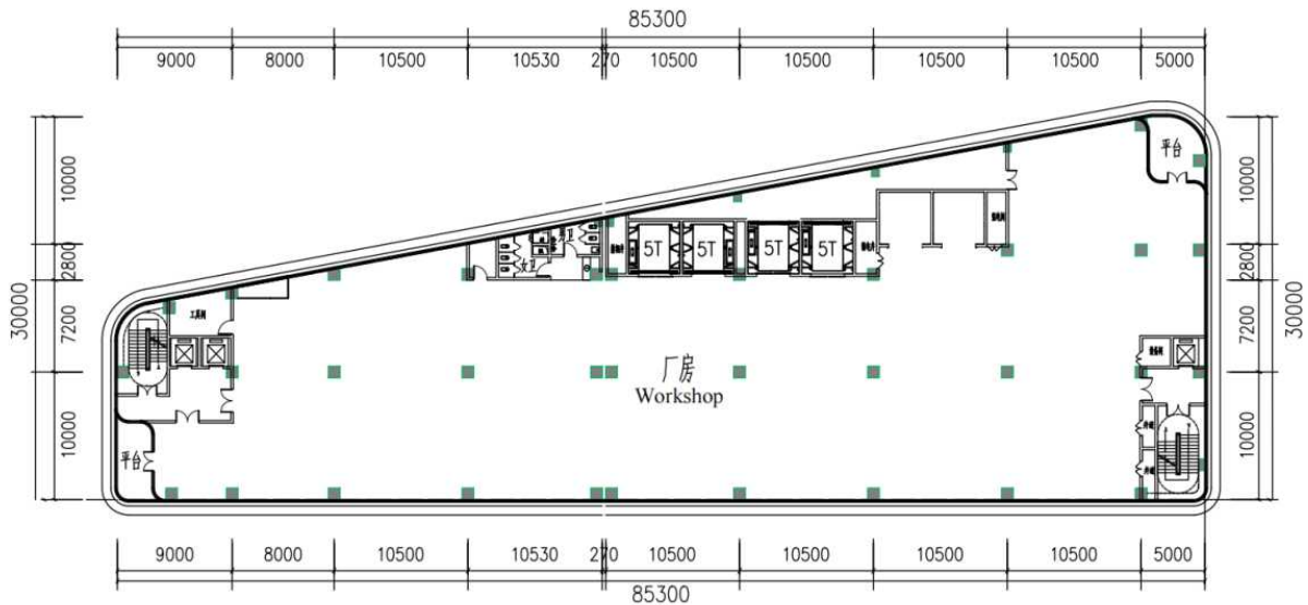
二层~七层平面图 2 nd ~7 th Floor Layout
